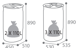
3-way freestanding sackholder
